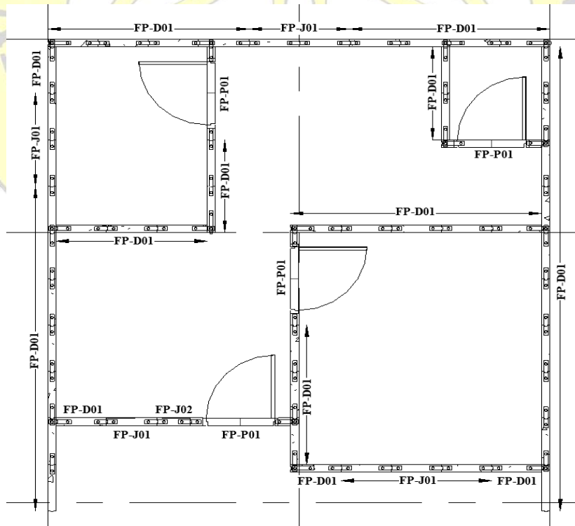
Denah Panel Model 2
