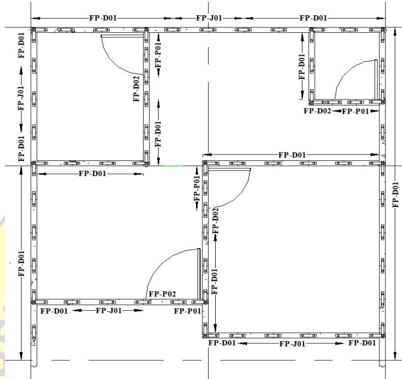
Denah Panel Model 1
