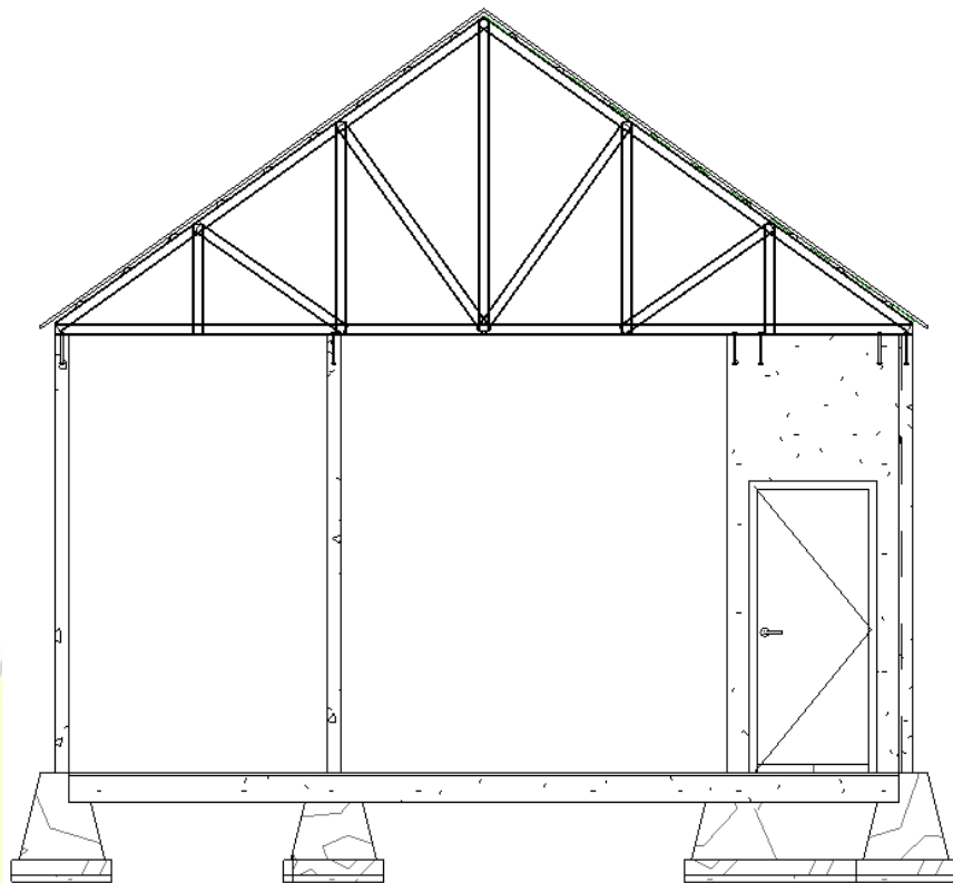
Potongan Model 2
