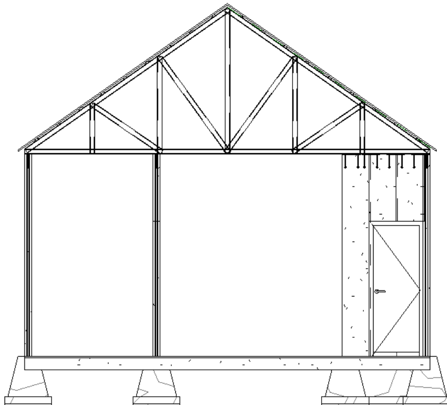
Potongan Model 1
